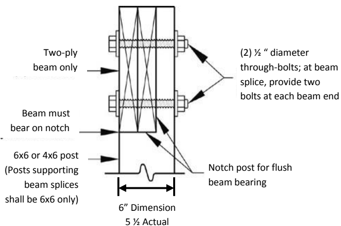
Notched Post
