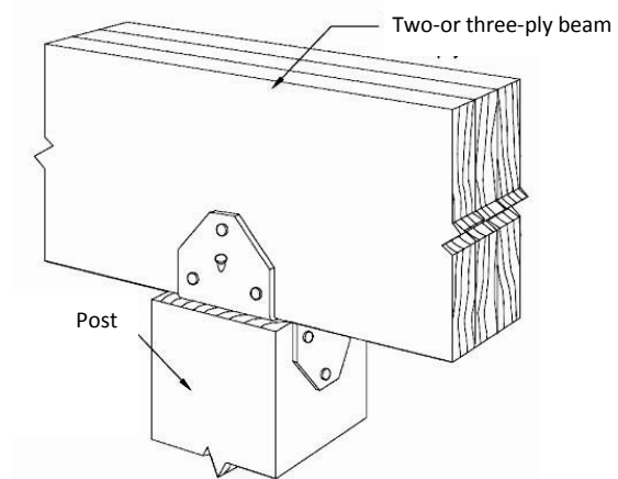
Post Cap
